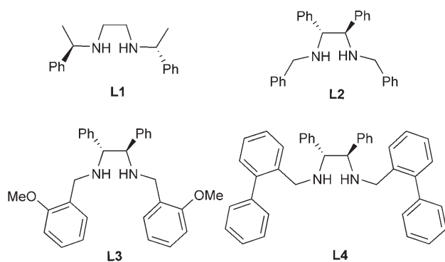
Figure 1. ( R,R )-Ebpe ( L1 ) and chiral diamine ligands ( L2–L4 ) derived from ( R,R )-dpen.
