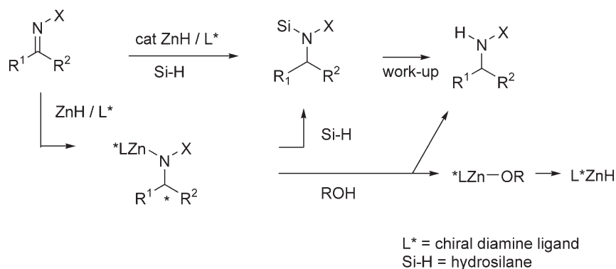
Scheme 1. Presumed reaction pathway for Zn-catalyzed reduction of imines.
